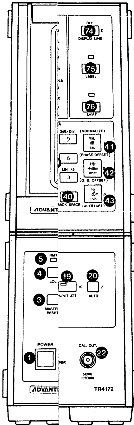
Fig. 3-2 Front panel
